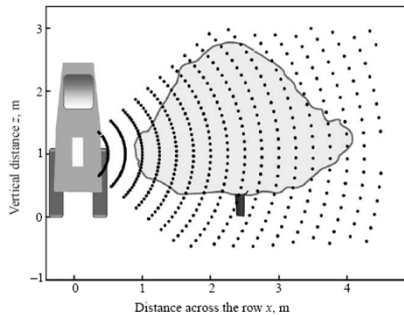
Fig. 3. Diagram showing the full grid pattern of contiguous elemental sampling volumes relative to the LIDAR origin.
